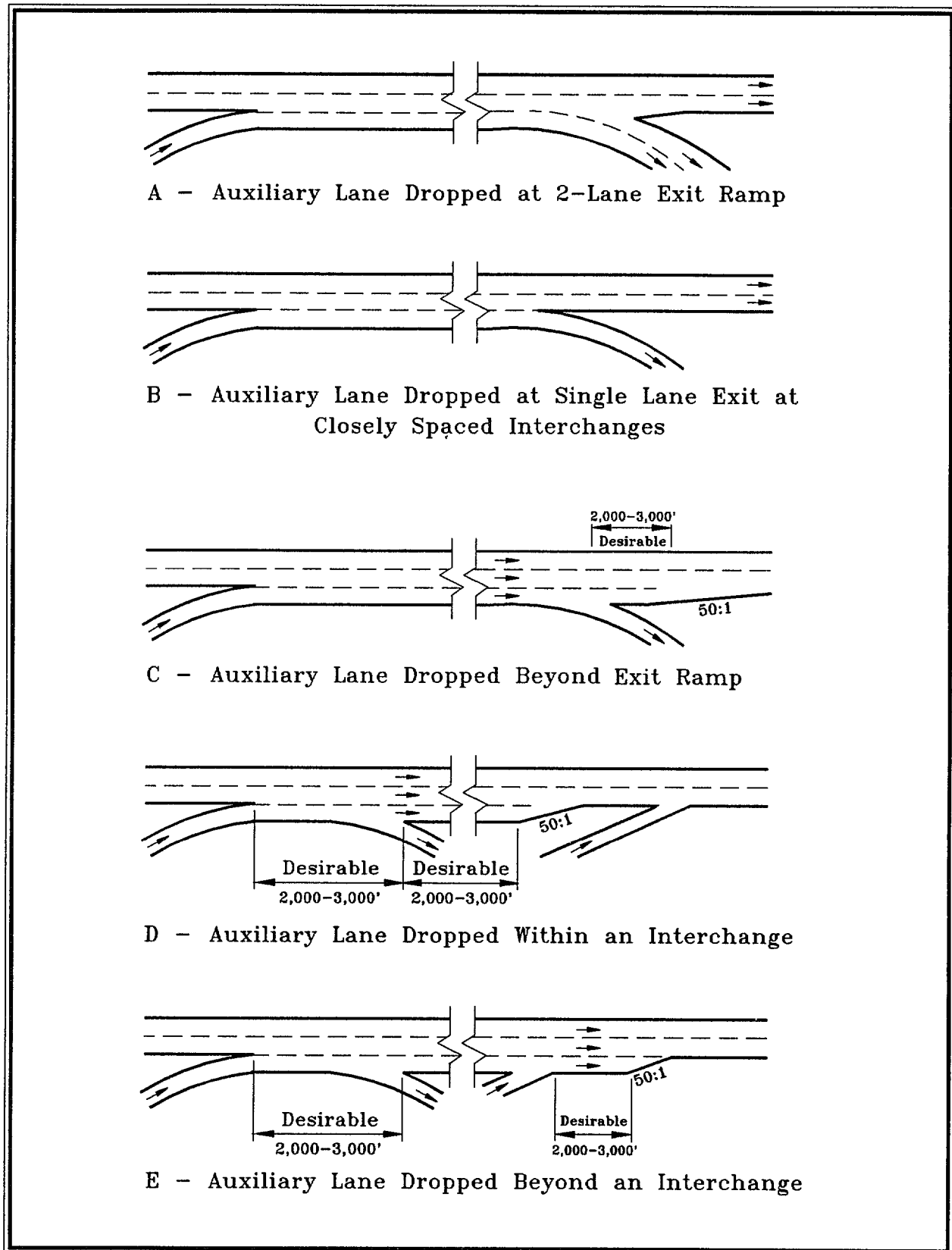
Figure 3-7. Alternatives for Dropping Auxiliary Lanes
