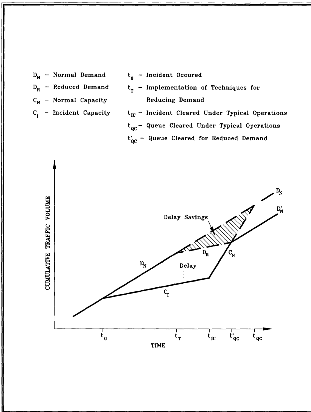
Figure 9-5. Incident Delay for Reduced Demand
