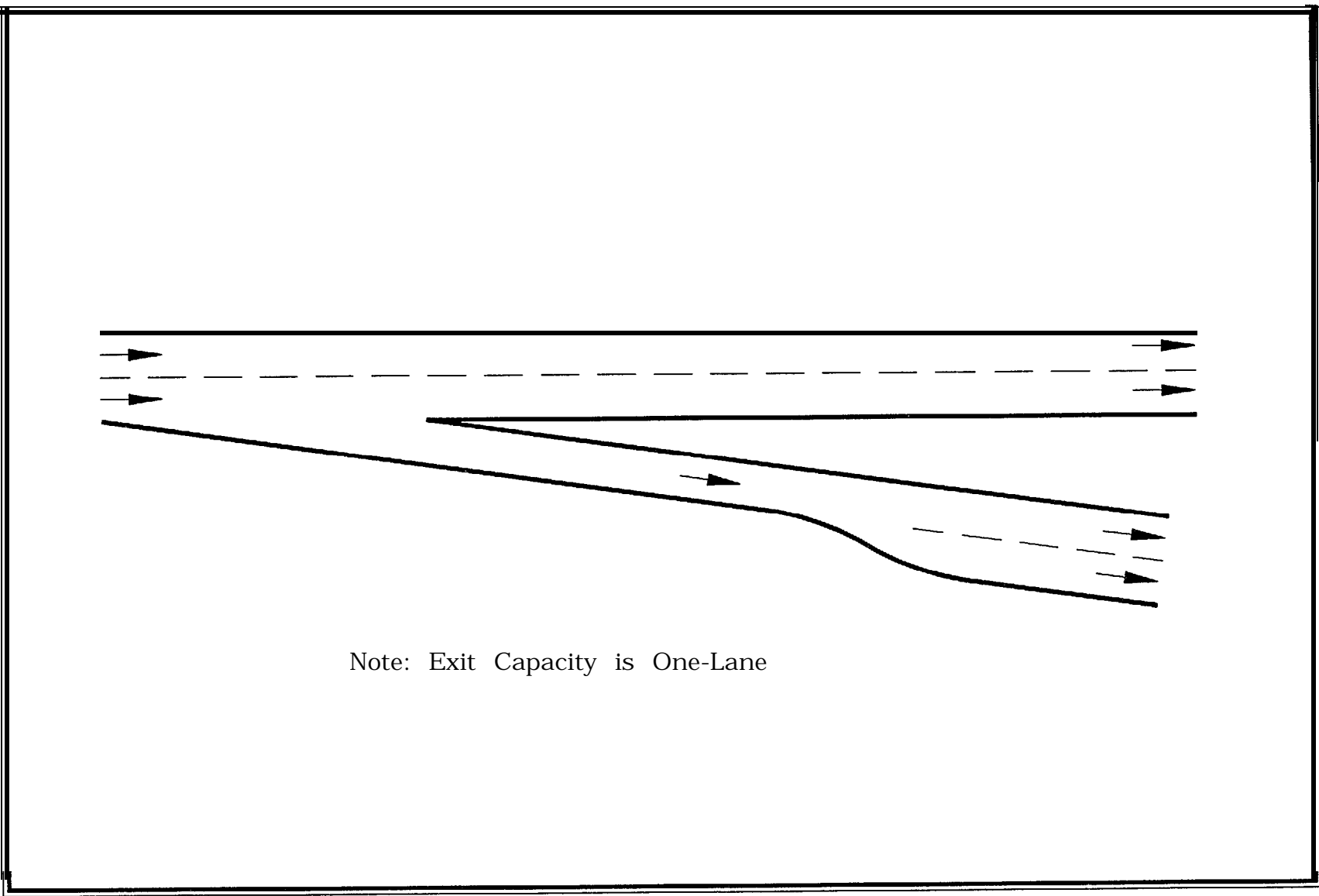
Figure 3-16. Lane Balance for Single Lane Transition to Two-Lane Exit Ramp
