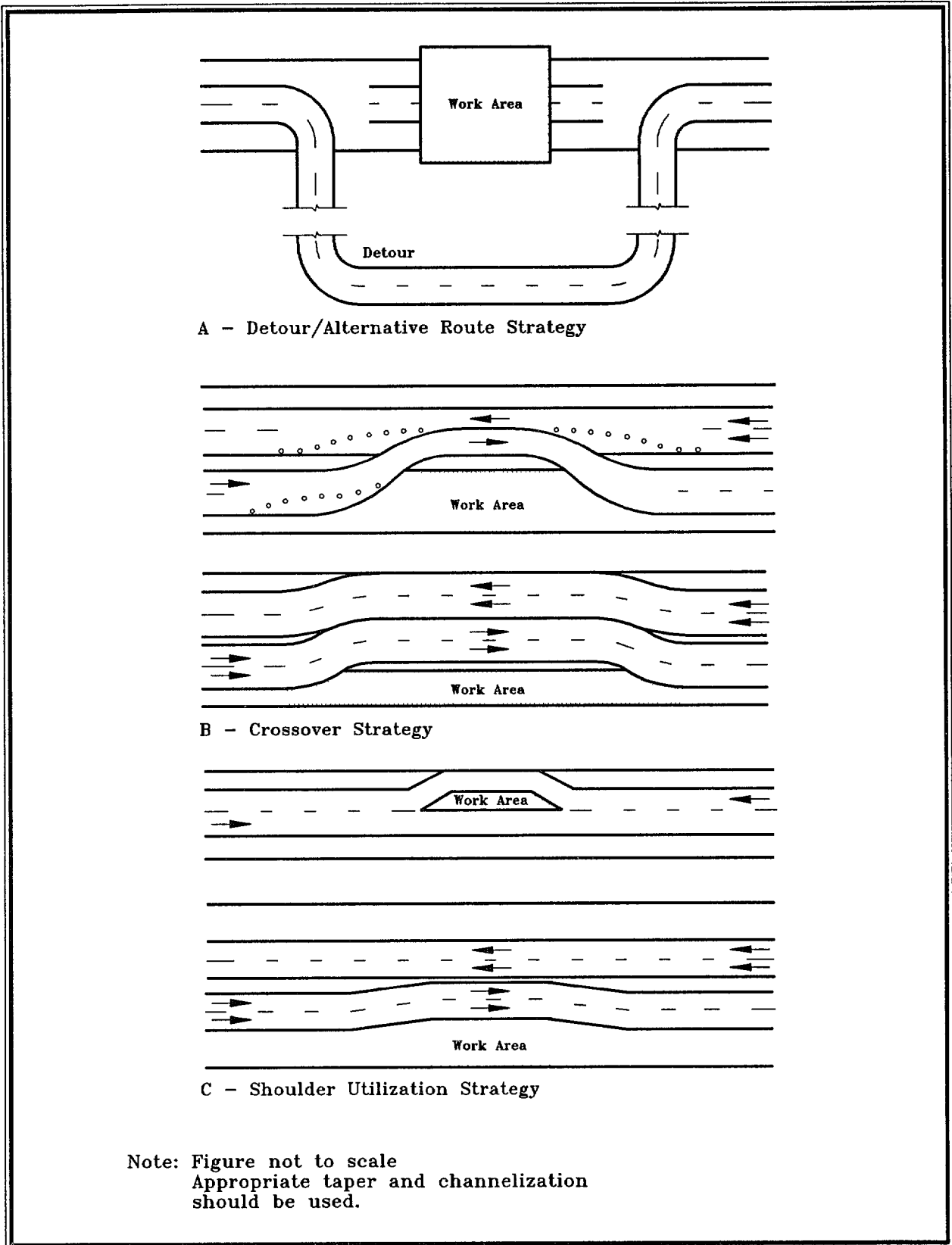
Figure 5-3. Other Management Strategies
