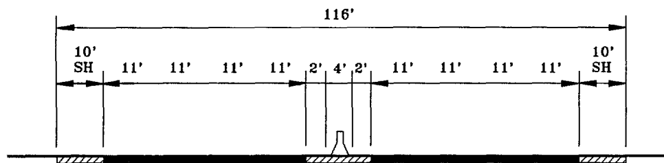
B - After, Restriped for Added Capacity
