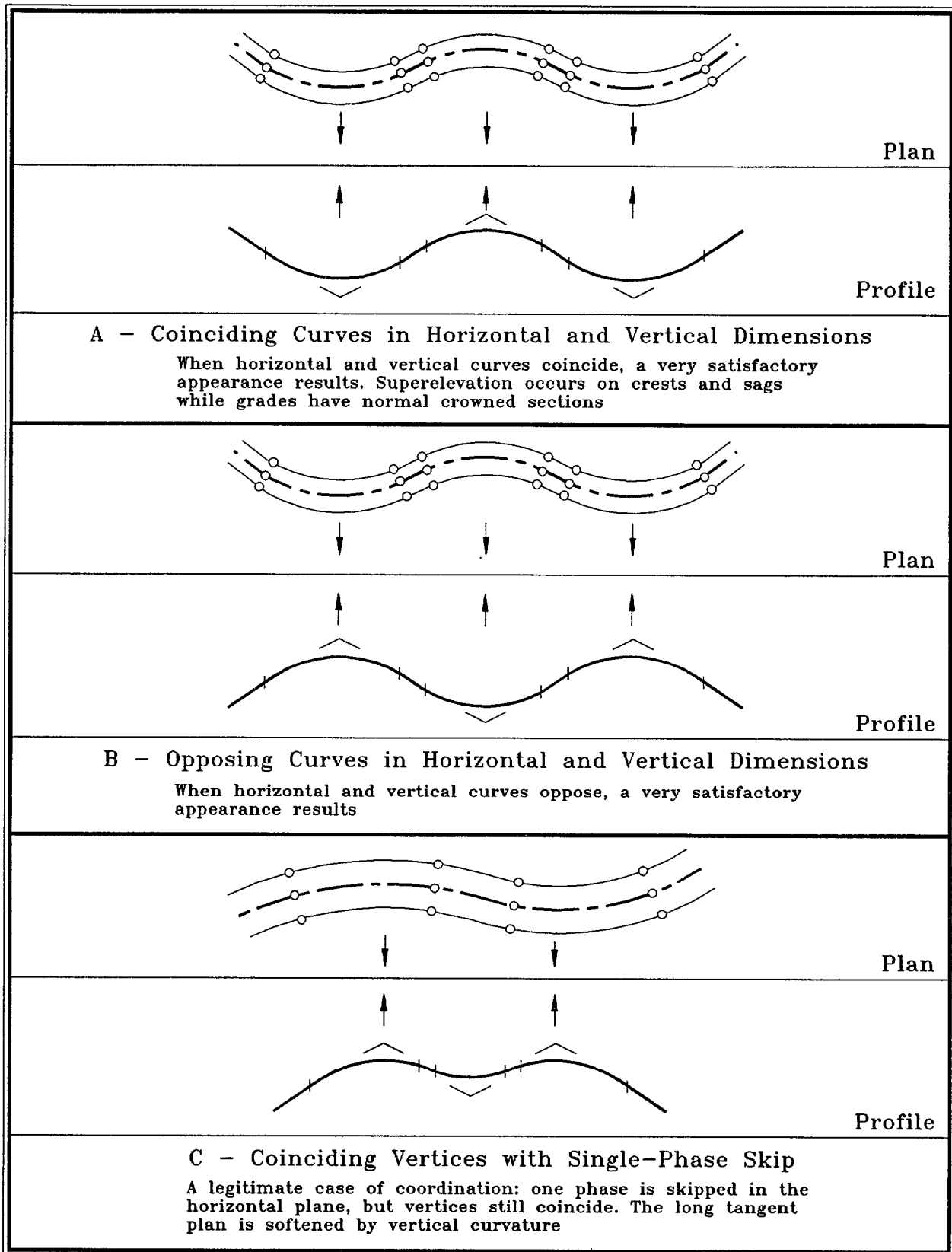
Figure 3-18. Coordination of Horizontal and Vertical Alignment
