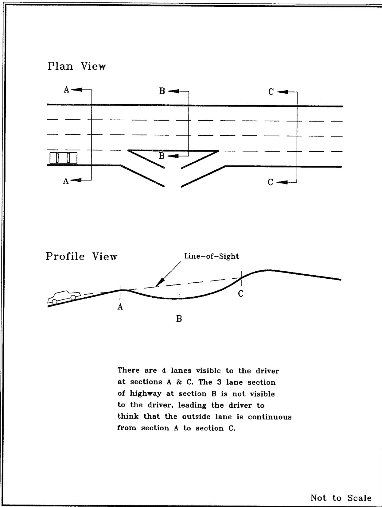
Figure 1-5. Deceiving Sight Distance Example
