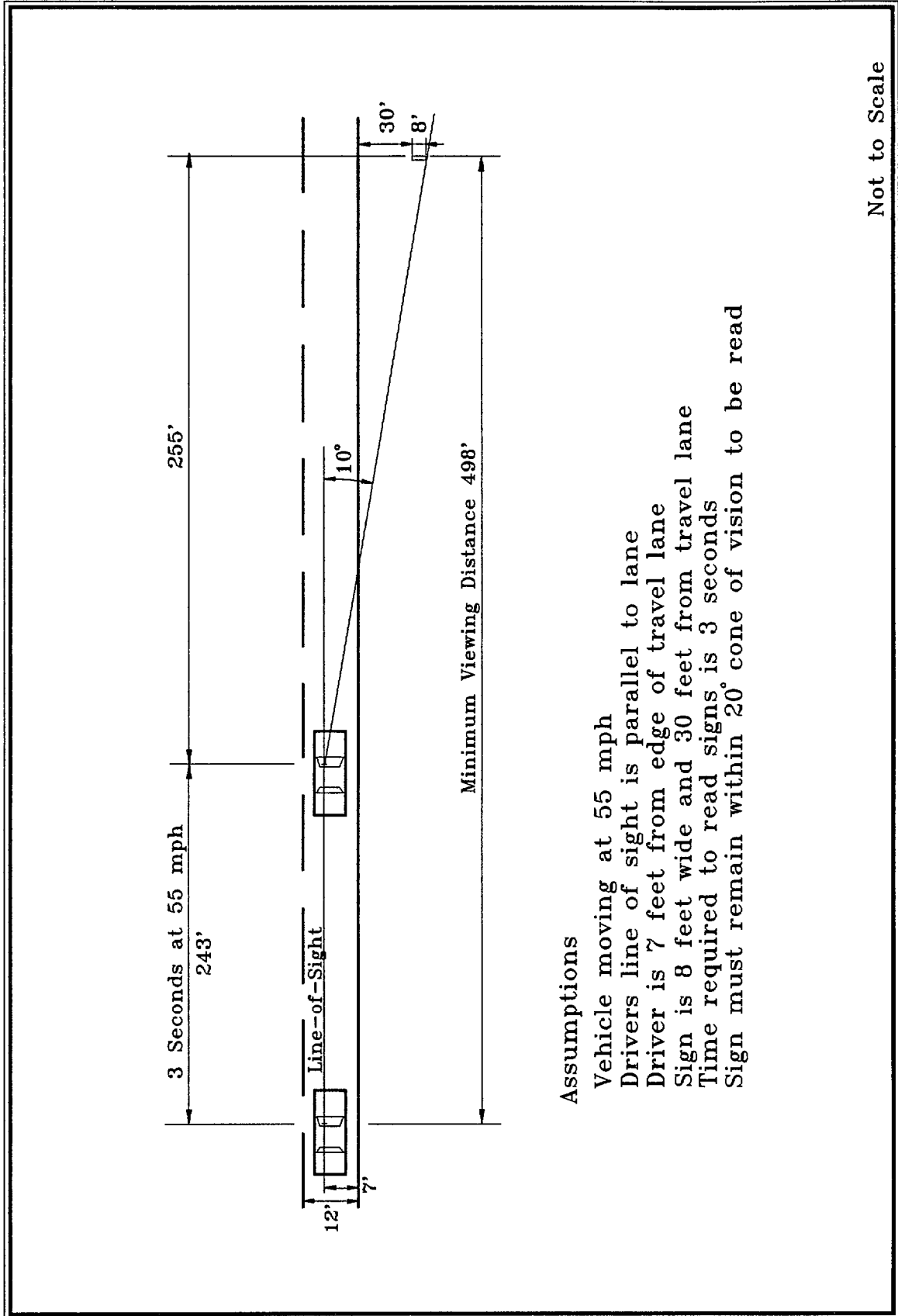
Figure 1-3. Sign Location and Cone of Vision
